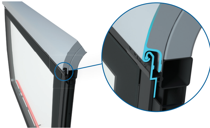
Structure Integrated Hinge
